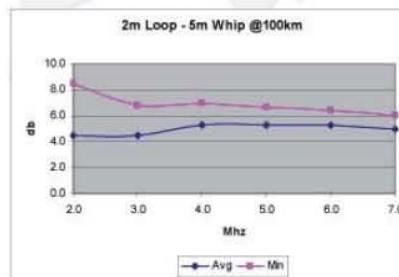
2m Half-loop Antenna
