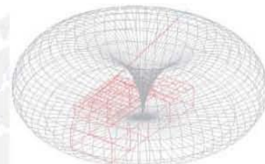
5m Whip Antenna
